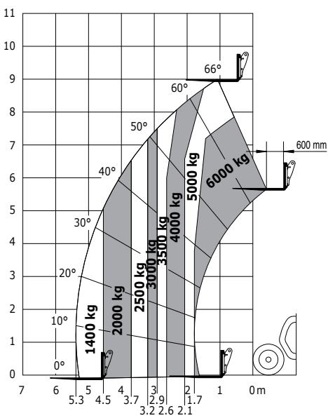
Industrial load chart standard EN1459 A Machines on tyres with forks
